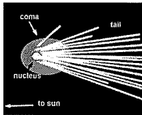
FIGURE 6 Graphic demonstrating the many features of a bright comet. Note: tail is opposite sun; Note: tail streamers at 11 O' and 2:30 positions are dust trailing tails (anti-tail).
